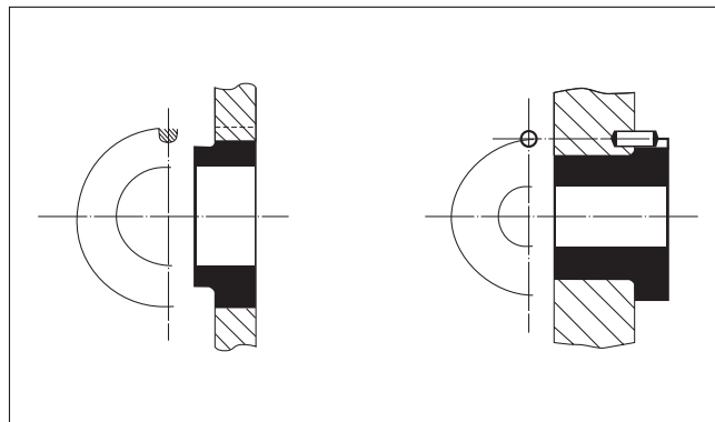
Protection against rotation with plain pin in the unloaded part of a carbon body
